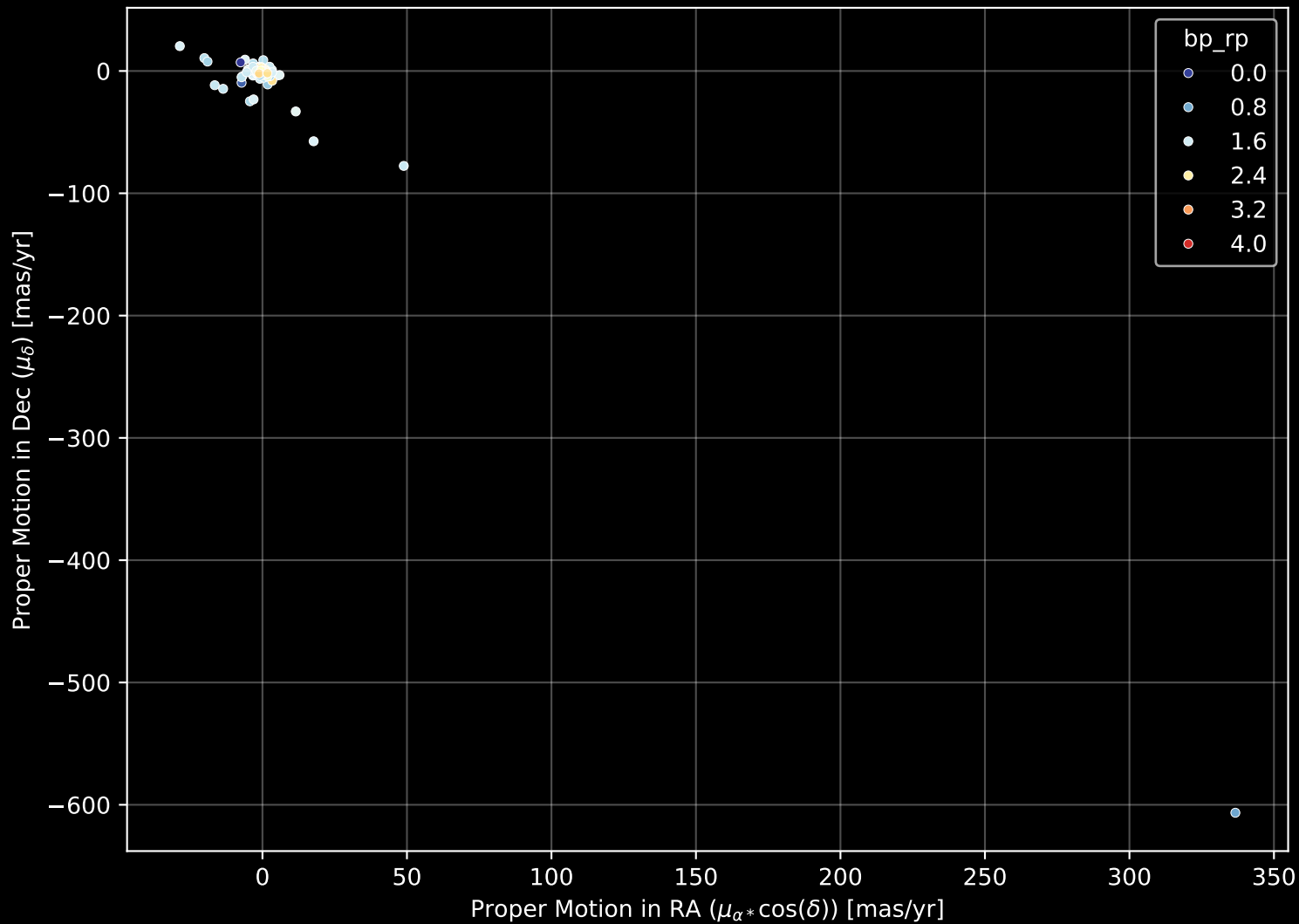
APOGEE DR17 Field: [214+00] Proper Motion Diagram (n= 377)
