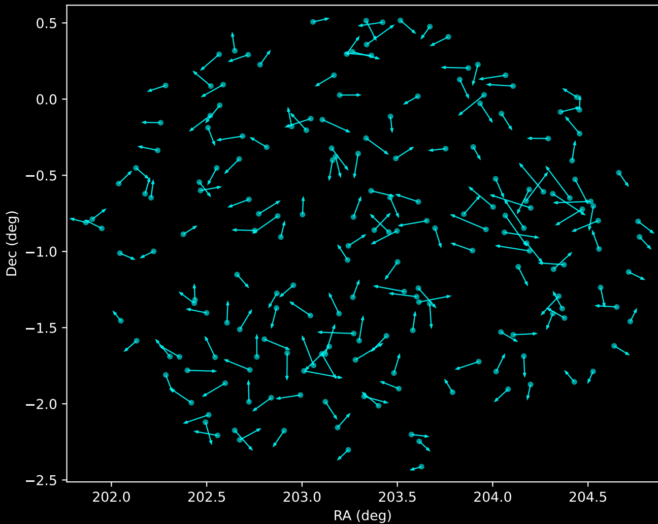
APOGEE DR17 Noise Stream Proper Motion Vectors (n=192)
