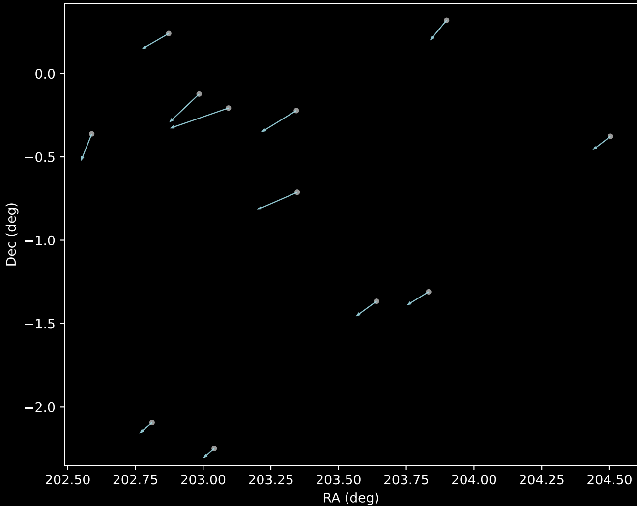
APOGEE DR17 Cluster 19 Proper Motion Vectors (n=12)
