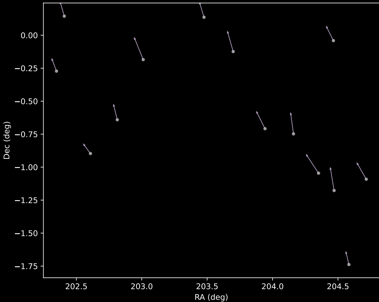
APOGEE DR17 Cluster 9 Proper Motion Vectors (n=14)
