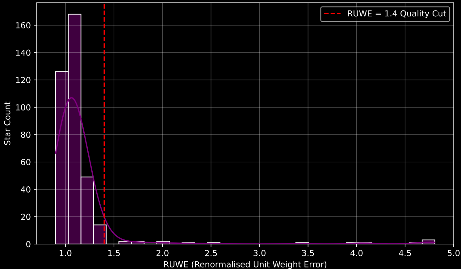
GAPOGEE DR17 Field [214+00] RUWE Distribution (n= 372)
