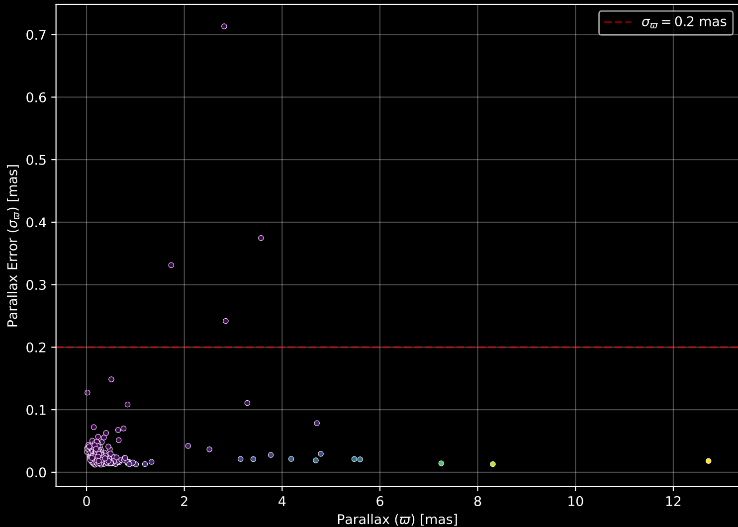
APOGEE DR17 Field: [214+00] Parallax Quality (n= 377)
