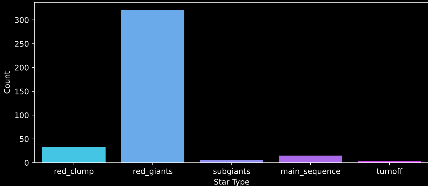
APOGEE DR17 Field: [214+00] Count plot of Star Type
