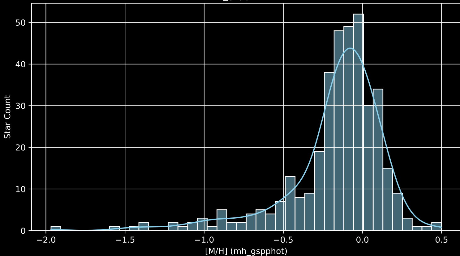
APOGEE DR17 Field: [214+00 [M/H] (mh_gspphot) (n= 374)
